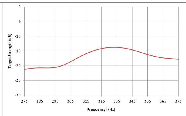
Narrowband Response of 325 kHz optimized (All TS figures \pm 2dB )
