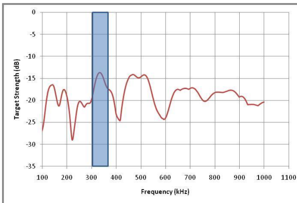
Broadband Response of 100mm SonarBell®
