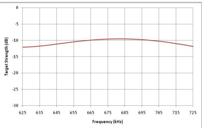
Narrowband Response of 675 kHz optimized (All TS figures \pm 2 dB)
