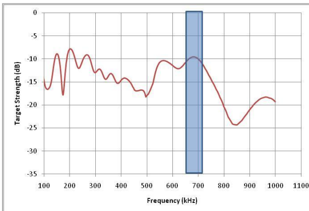
Broadband Response of 200mm SonarBell®
